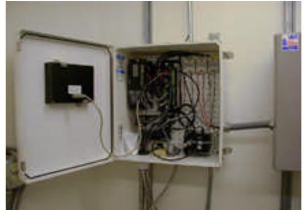
Inside view of the SCAD Control Unit enclosure. CR10X Unit, PS12LA Rechargeable Power Supply, Solid State Relays for pump control and COM310 Voice Phone Modem.
