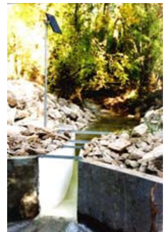
Box Elder Creek, 9" FRP Par shall Flume with attached 12" stilling well, instrumented with PT1830 DRUCK pressure transducer attached to a CR510 Data logger.
